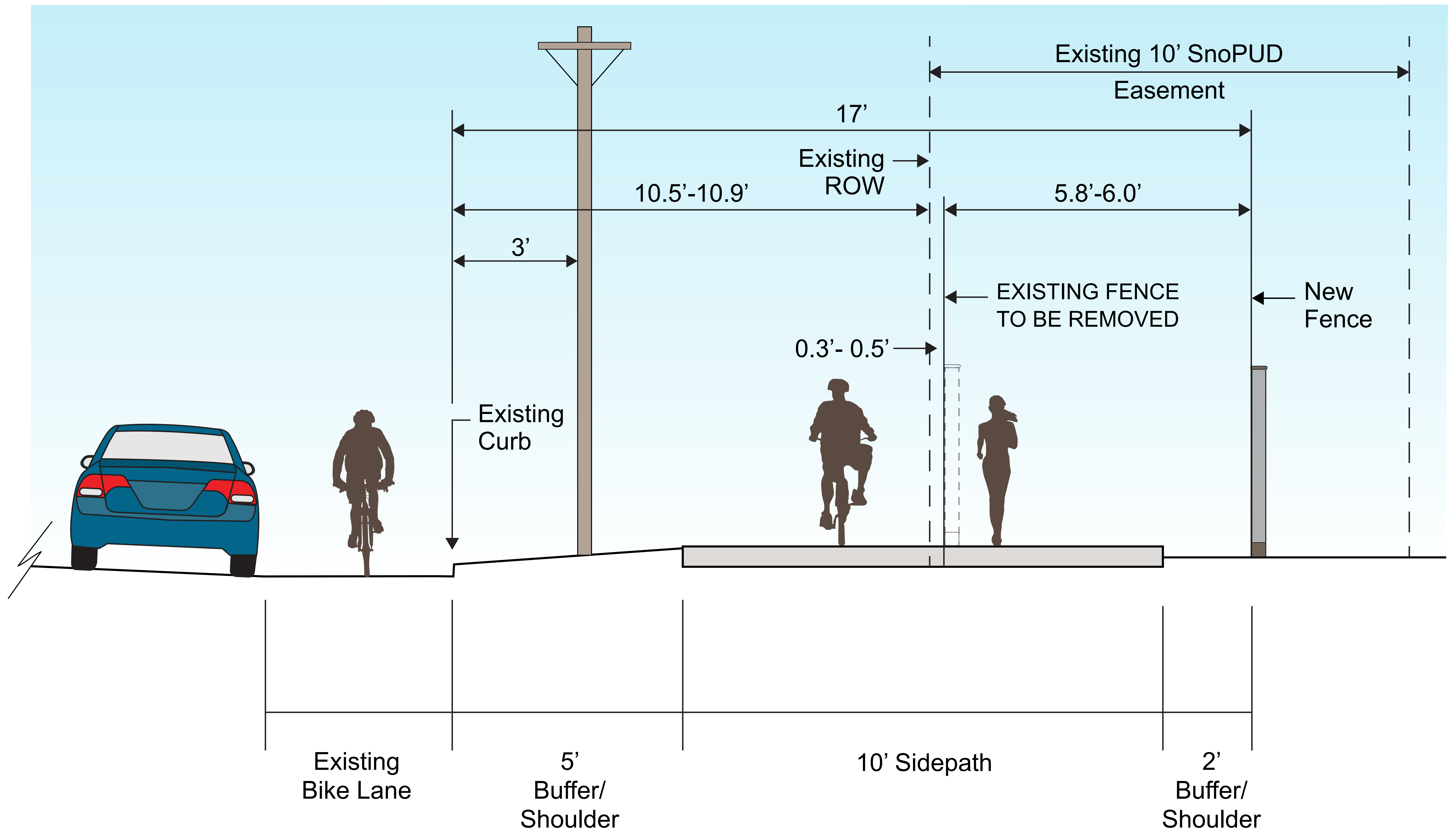
TYPICAL CROSS SECTION ADJACENT TO MURIEL'S LANDING
